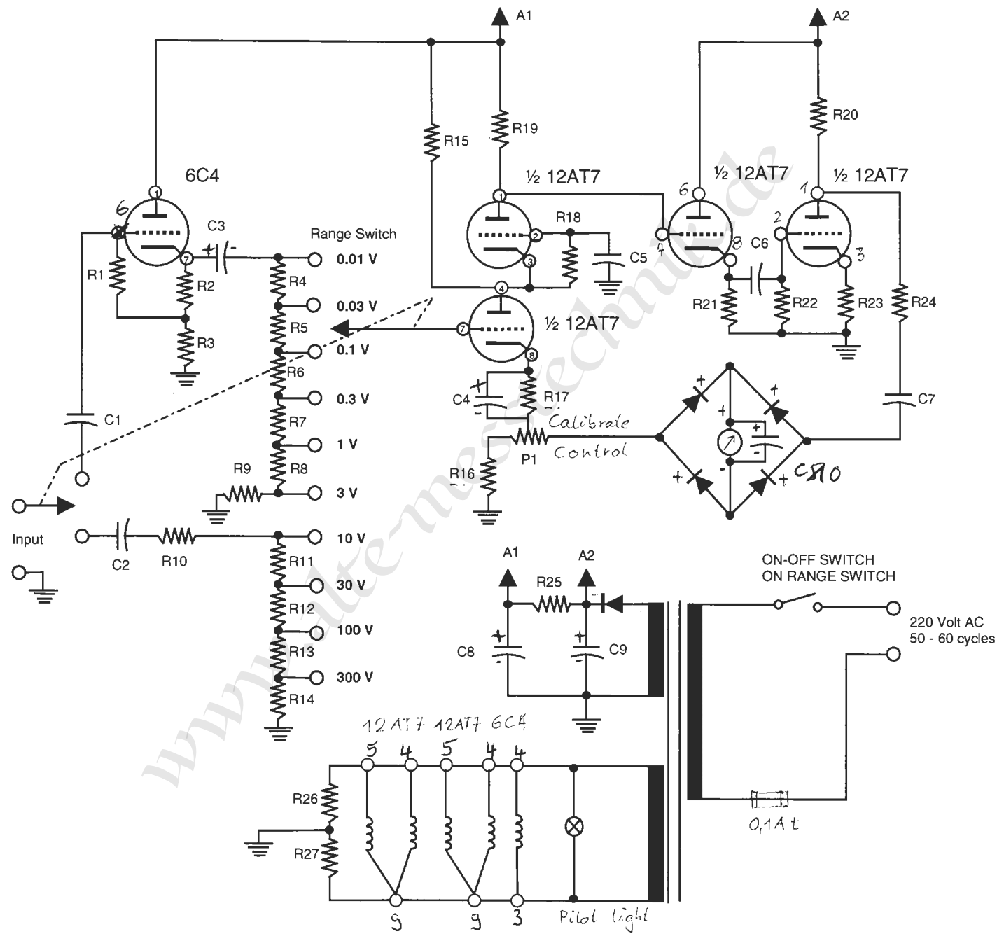
AV-3 Audio VTVM circuit diagram
